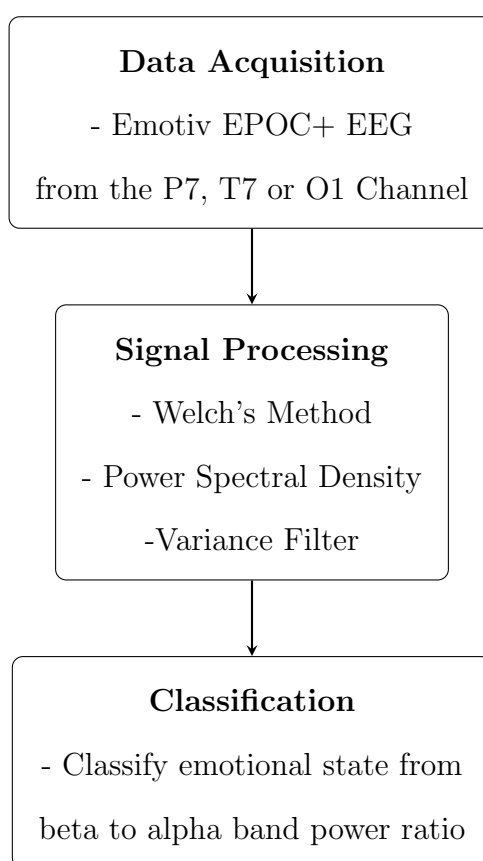
Figure 5.3: Workflow of EEG data analysis
